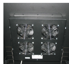
Image shows roof mounted Smart Net Fan Unit fitted in cabinet.
